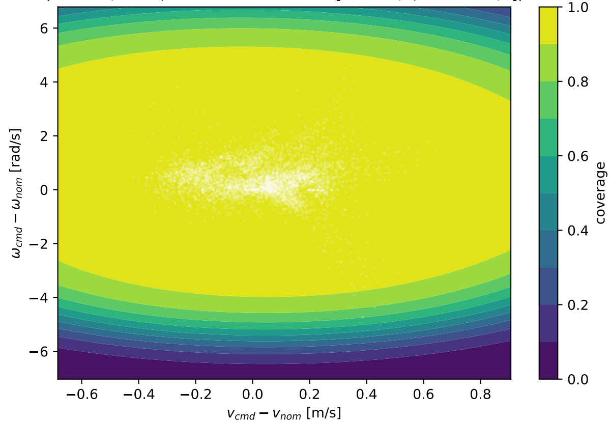
Residual coverage vs command offset (0 = off / OOD; state fixed at mean [0.64 m/s, -0.07 rad/s])
